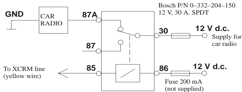
Figure 4: Car Radio Muting CRM
