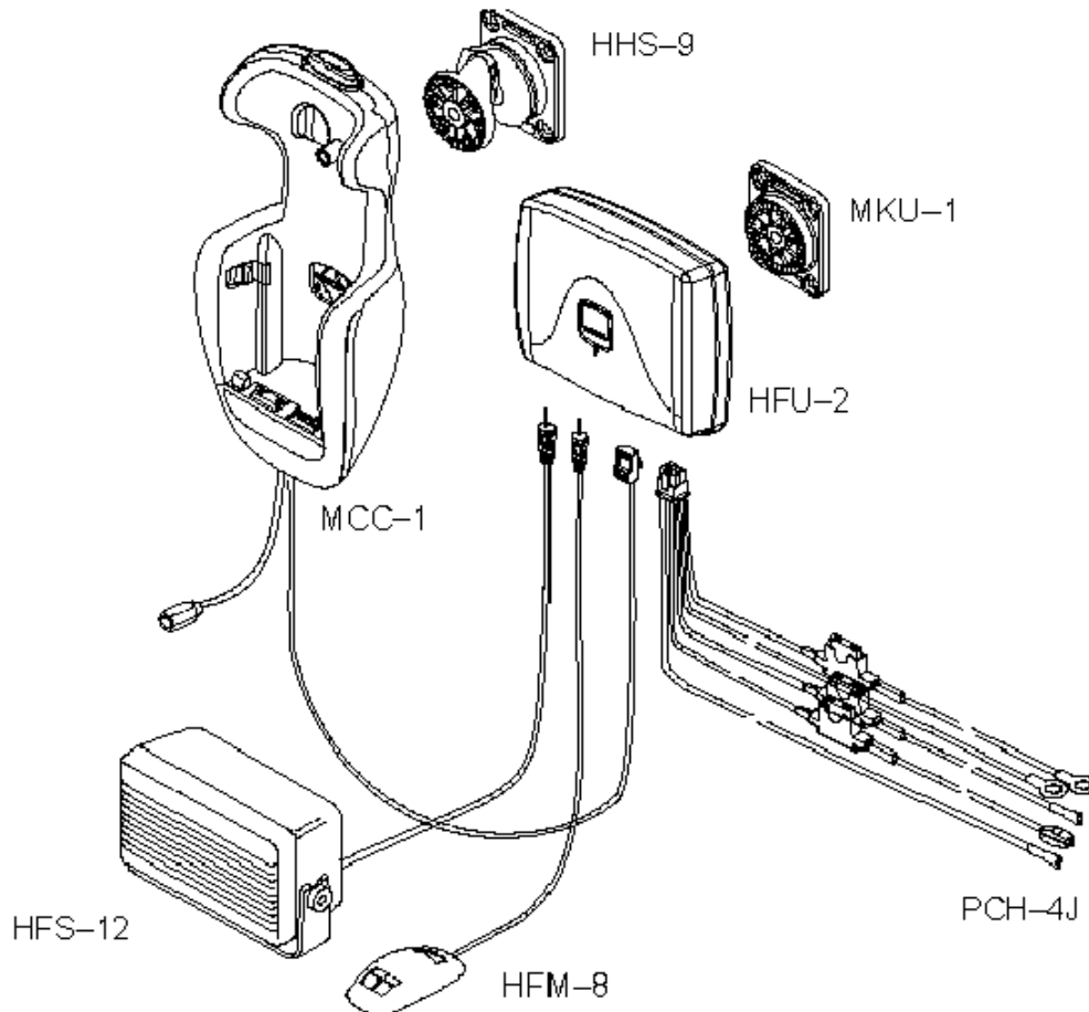
Figure 3: Equipment
